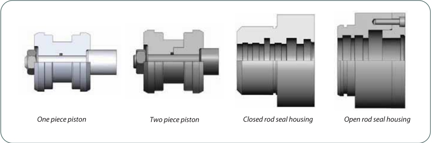
Sample gland cap and piston designs
